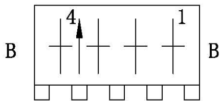
M7239R-4-BB-3 (2)
