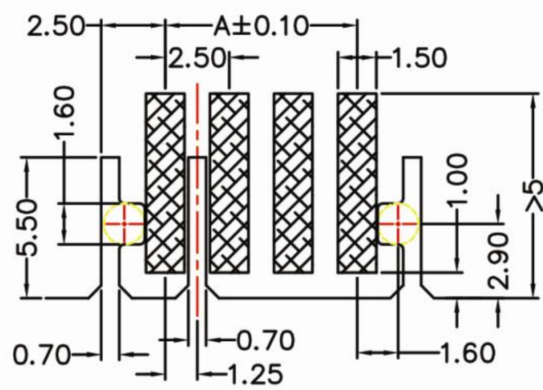
P. C. Board layout
