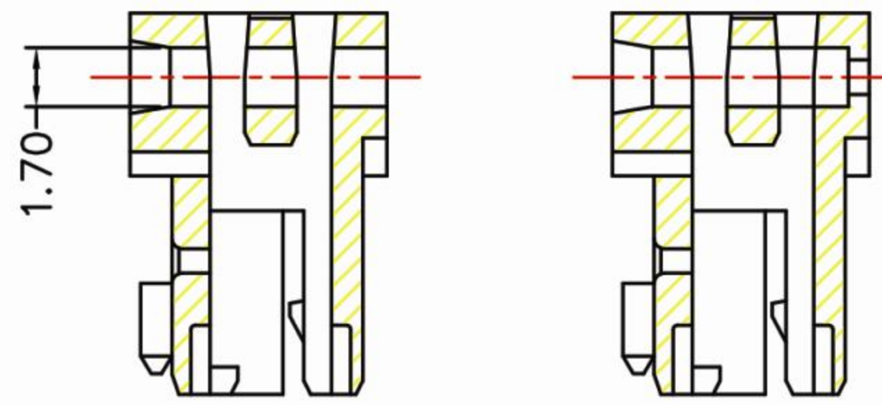
SECTION: B-B
